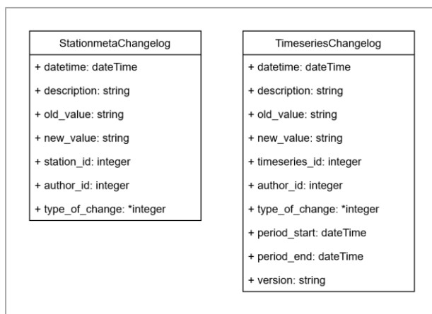
Figure 5: Structure of StationmetaChangelog and TimeseriesChangelog records. Each Stationmeta or Timeseries entry may contain 1..N Changelog entries.
