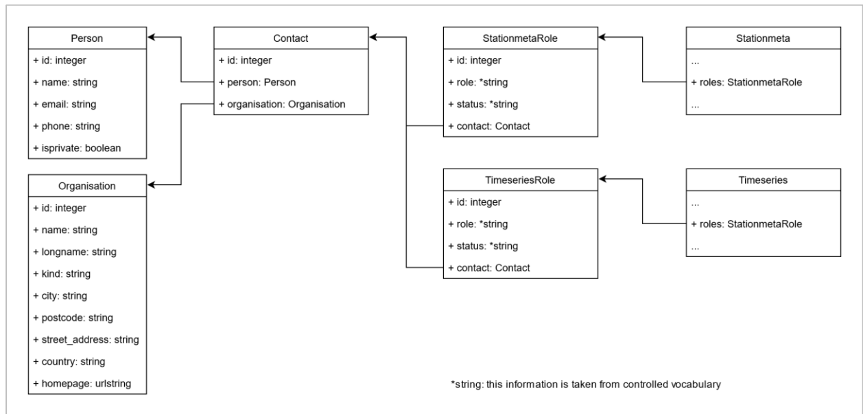
Figure 3: TOAR database model for recording roles of people and organisations in the data creation and curation process
